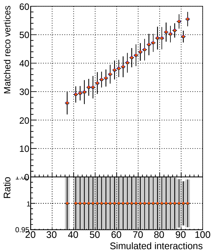
MatchedRecoVtx_vs_GenVtx
