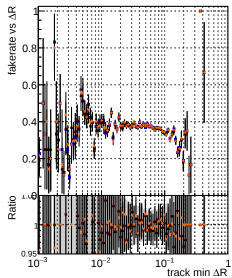
Legend for Fake rate vs \Delta R : DOM (black line) REDO (blue line) signal (orange line) option0 (red line) option1 (green line) option2 (purple line)
