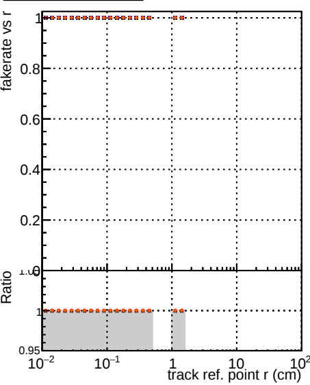
Fake rate vs v Legend DOM IT original REDO Line Blue Red Black Black Star Blue Red Black Black Star Blue Red Black Black Star Blue Red Black Black
