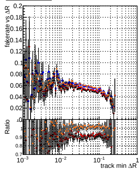
Legend for Fake rate vs \Delta R : DOM (black line) TT (blue line) original (red line) REDO (orange line) options0 (grey line) options1 (light blue line) options2 (light orange line)
