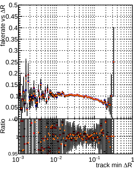
Fake rate vs \Delta R(\text{track, jet}) Legend: DOM TT original REDO DOM TT original option0 DOM TT original option2
