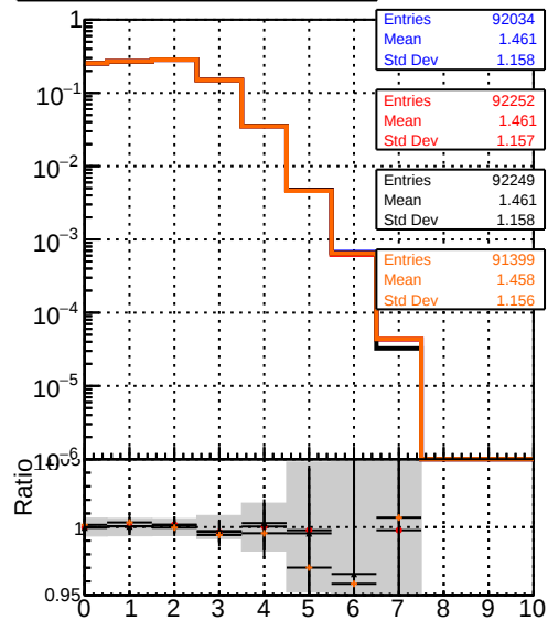
mean hit DQM_TT originalREDO DQM_TT original_option0 DQM_TT original_option1 DQM_TT original_option2
