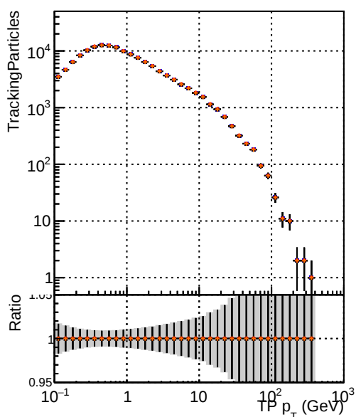
Legend for all plots: DQM TT originalREDO (blue circles) DQM TT original_option0 (red diamonds) DQM TT original_option1 (black triangles) DQM TT original_option2 (orange stars)
