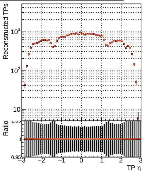
Legend for all plots: DQM TT originalREDO (blue circles) DQM TT original_option0 (red diamonds) DQM TT original_option1 (black triangles) DQM TT original_option2 (orange stars)
