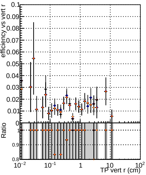
Efficiency vs vertpos DOM TT originalREDO DOM TT original_option0 DOM TT original_option1 DOM TT original_option2
