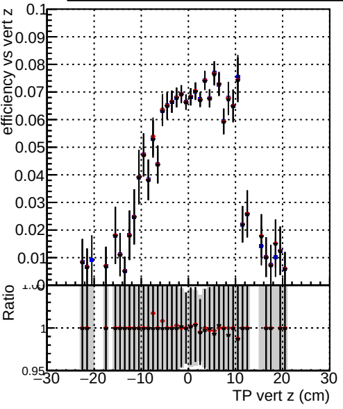
Efficiency vs TP vert z (cm) Legend: DQM_TT_CKF_ORIG (Blue squares) DQM_TT_CKFLowPtT_ORIG (Red circles) DQM_TT_CKFLowPtT_MODIF (Black stars)
