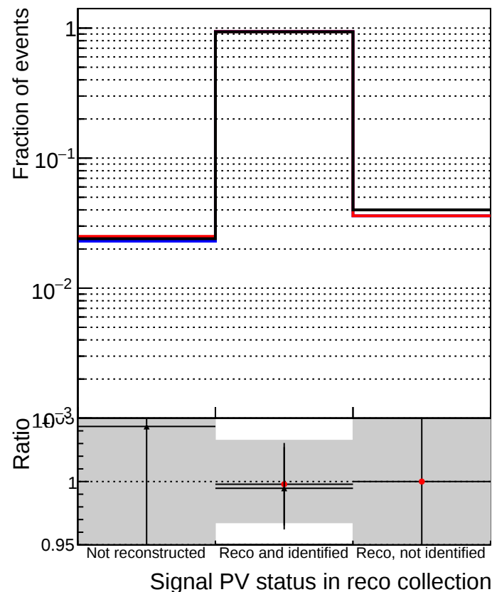
TruePVLocationIndexInRecoVertexCollectionCumulative
