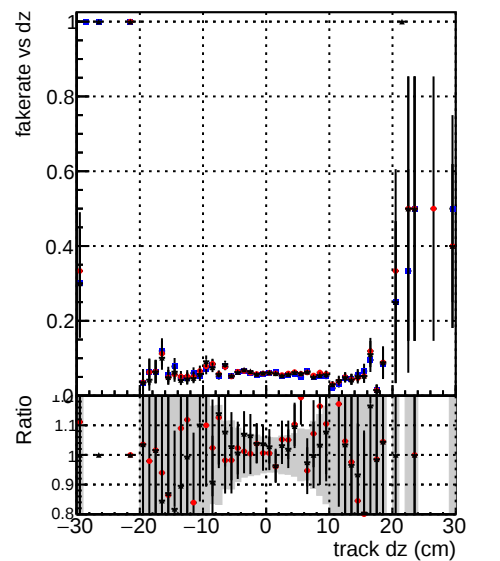
Fake rate vs d
