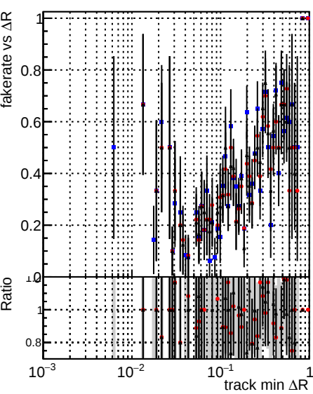
Fake rate vs \Delta R(\text{track, jet}) Legend: DOM TT CKF_ORIG (blue dots) DOM TT CKFLowPt_ORIG (red dots) DOM TT CKFLowPt_MODIF (black dots)
