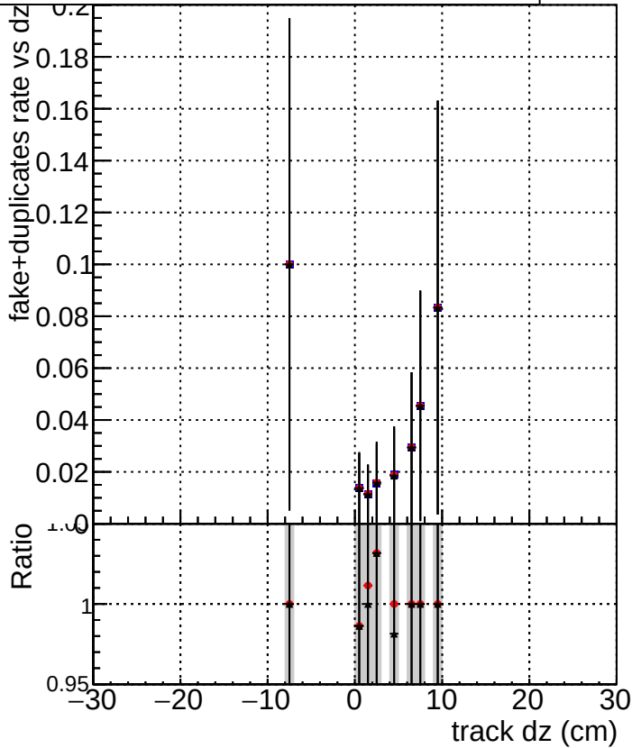
Legend: DQM_TT_CKF_ORIG (Blue square) DQM_TT_CKFLowPtT_ORIG (Red circle) DQM_TT_CKFLowPtT_MODIF (Black triangle)
