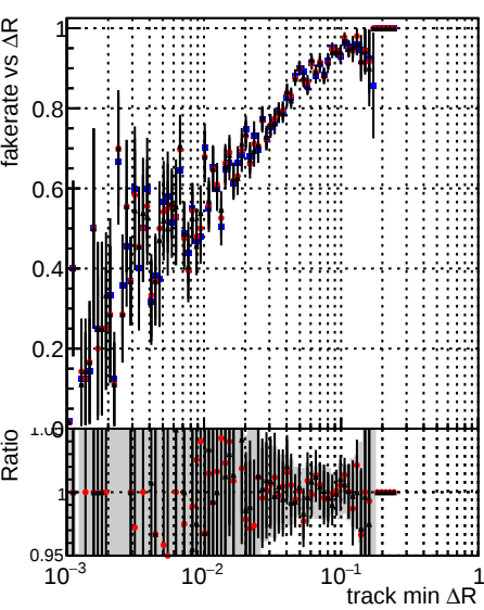
Legend: DQM TT CKF_ORIG (black line with blue dots), DQM TT CKFLowPt_ORIG (red line with red dots), DQM TT CKFLowPt_MODIF (black line with black dots)
