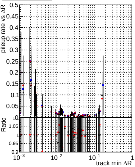
Legend: DQM TT CKF_ORIG (black line with blue dots), DQM TT CKFLowPt_ORIG (red line with red dots), DQM TT CKFLowPt_MODIF (black line with black dots)
