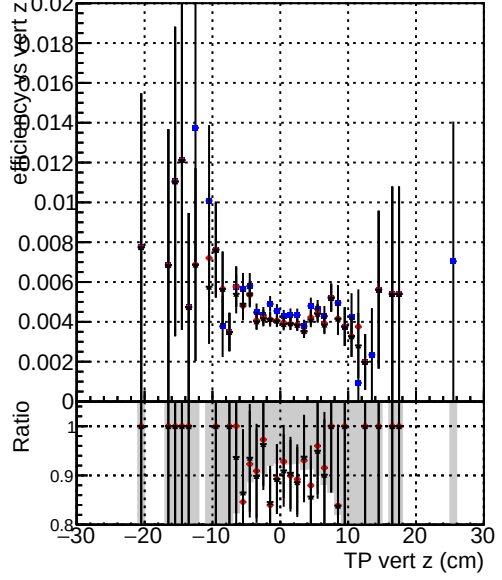
Efficiency vs. TP vert z (cm) Legend: - DQM_TT_CKF_ORIG (blue circles) - DQM_TT_CKFlowPIT_ORIG (red circles) - DQM_TT_CKFlowPIT_MODIF (black circles)
