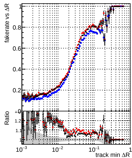
Legend for Fake rate vs \Delta R , Duplicates Rate vs \Delta R , and Pileup rate vs \Delta R : DOM TT CKF_ORIG (blue diamonds) DOM TT CKFLowPtQ_ORIG (red circles) DOM TT CKFLowPtQ_MODIF (black crosses)
