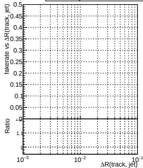
Legend for Fake rate vs \Delta R , Duplicates Rate vs \Delta R , and Pileup rate vs \Delta R : DOM TT CKF_ORIG (blue diamonds) DOM TT CKFLowPtQ_ORIG (red circles) DOM TT CKFLowPtQ_MODIF (black crosses)
