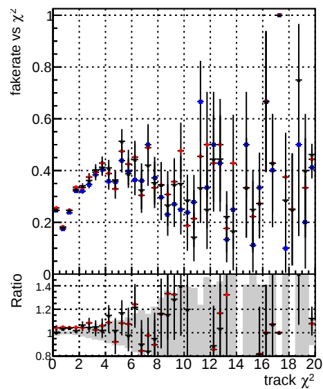
Fake rate vs. DOM TT CKF ORIG DOM TT CKF LOWP TO ORIG DOM TT CKF LOWP TO MODIF Blue Red Black
