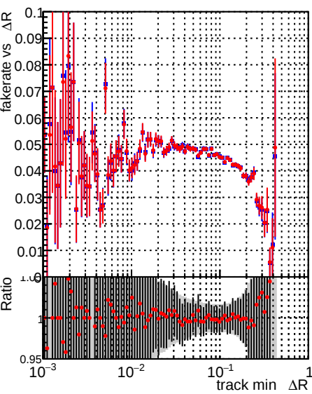
Fake rate vs \Delta R (track, jet) DQM_legacy_noSel DQM_legacy_fit_noSel
