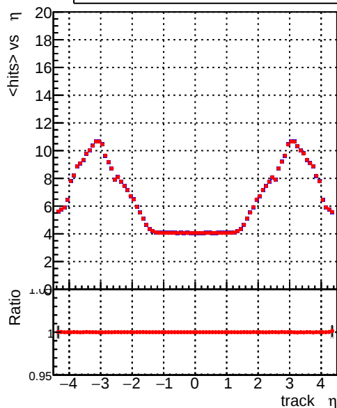
mean hits vs \eta Legend: DQM_7571_noSel (blue line), DQM_7572_noSel (red line)
