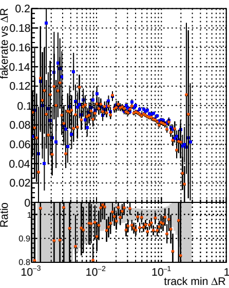
Fake rate vs \Delta R (track, jet) Legend: DOM CKE TTbar mktfit TTbarPU BNN mktfit100
