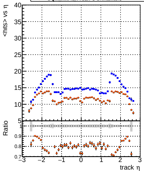
mean hit DQM_CKFit_TTbar DQM_mkFit_TTbarPU-updated DQM_mkFit_TTbarPU-DNNsqcd100 DQM_mkFit_TTbarPU-DNNalliters
