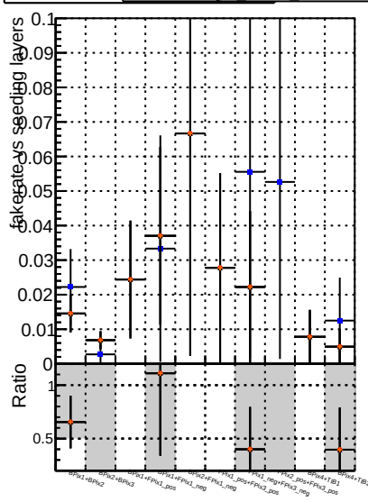
Fake rate vs. DOM GKE TTher TTher+BU updated 100
