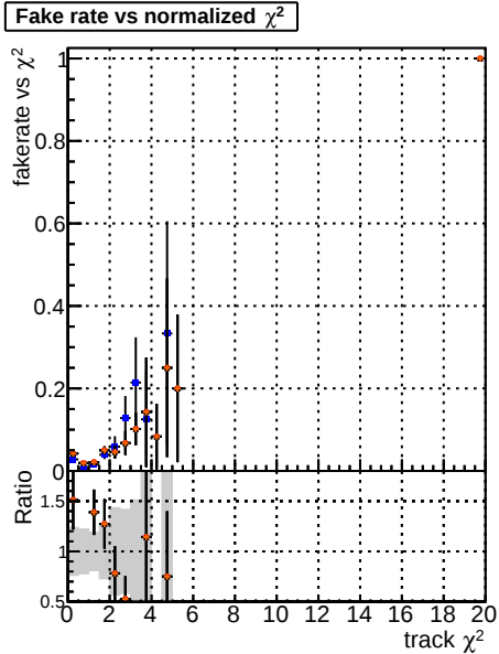
Fake rate vs. Legend: DOM GKE TTher DOM MR TTBar PU updated 100 DOM MR TTBar PU BNN 100
