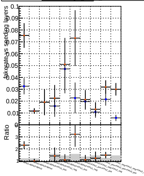
Fake rate vs. Legend: DOM GKE TTher DOM MR TTBar PU updated 100 DOM MR TTBar PU BNN 100
