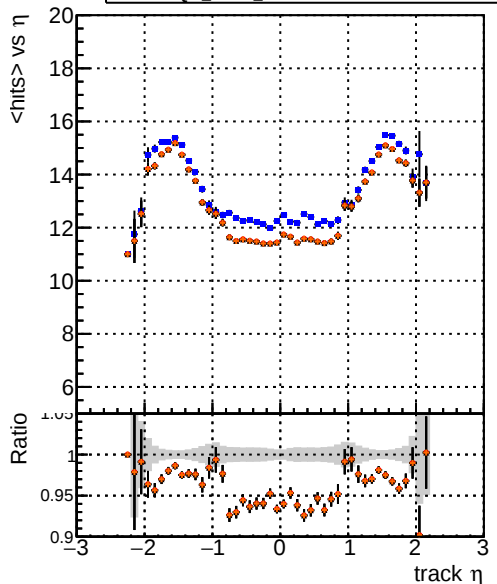
Legend: DQM_CKF_TTbar (blue line), DQM_mkFit_TTbarPU-updated (red line), DQM_mkFit_TTbarPU-DNNsqcd100 (black line), DQM_mkFit_TTbarPU-DNNalliters (orange line) mean hit
