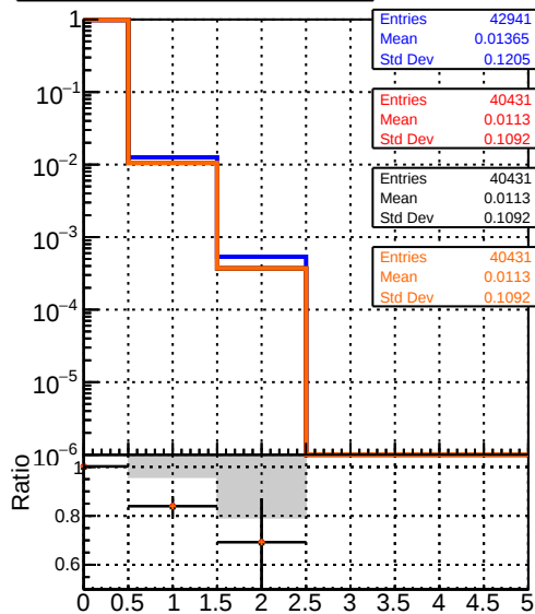
mean hit — DQM_CKF_TTbar — DQM_mkFit_TTbarPU-updated — DQM_mkFit_TTbarPU-DNNsqcd100 — DQM_mkFit_TTbarPU-DNNalliters
