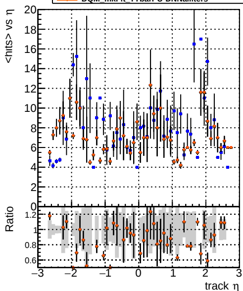
— DQM_CKF_TTbar — DQM_mkFit_TTbarPU-updated — DQM_mkFit_TTbarPU-DNNsqcd100 — DQM_mkFit_TTbarPU-DNNalliters mean hit
