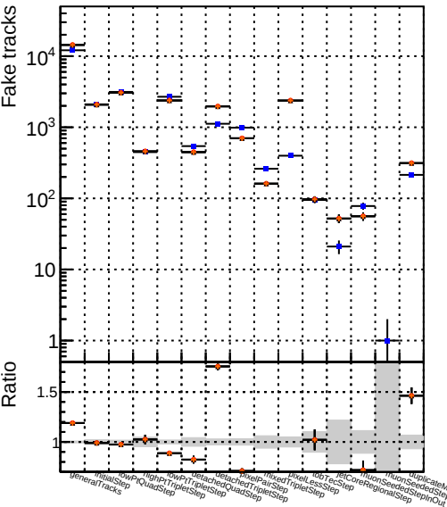
Number DQM_mkFit_TTbarPU-DNNsgcd100 DQM_mkFit_TTbarPU-DNNalliters
