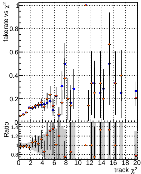
Fake rate vs. \chi^2 for different models and layers
