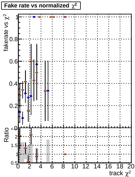
Fake rate vs. DOM GKE TTher DOM+GKE TTher+GKE DOM+GKE+TTher
