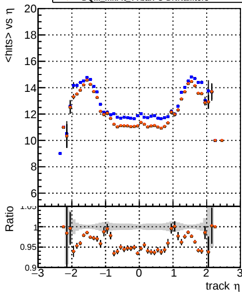
mean hits — DQM_CKF_TTbar — DQM_mkFit_TTbarPU-updated — DQM_mkFit_TTbarPU-DNNsqcd100 — DQM_mkFit_TTbarPU-DNNalliters
