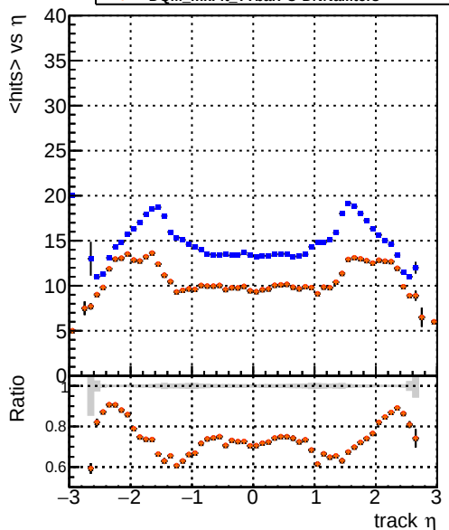
mean hit DQM_CKF_TTbar DQM_mckFit_TTbarPU-updated DQM_mckFit_TTbarPU-DNNsqcd100 DQM_mckFit_TTbarPU-DNNalliters
