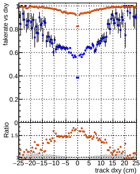
Legend for Fake rate vs dxy: DGM (orange line) SKE (blue line) TTbar (black line) TTbar+updated (black line) TTbar+NN (black line) TTbar+NN+NN (black line)
