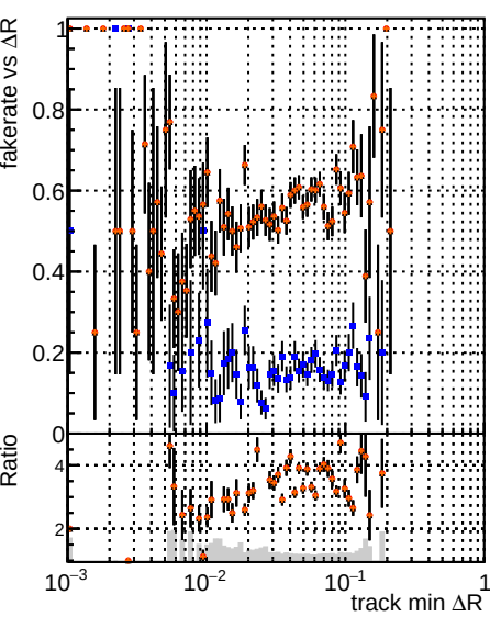
Fake rate vs \Delta R(\text{track, jet}) Legend: BQM CKE Ttbar BQM mktfit TtbarPU-updated BQM mktfit TtbarPU-BNN BQM mktfit TtbarPU-100
