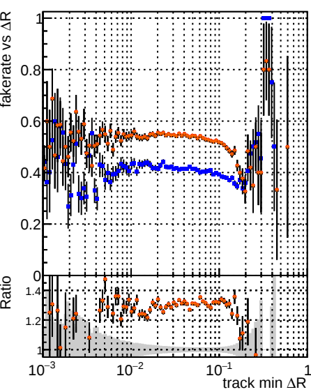
Fake rate vs \Delta R(\text{track, jet}) Legend: DOM CKE Tbar DOM mktfit Tbar DOM mktfit Tbar PU-updated DOM mktfit Tbar PU-BNN DOM mktfit Tbar PU-BNN 100 DOM mktfit Tbar PU-BNN 1000
