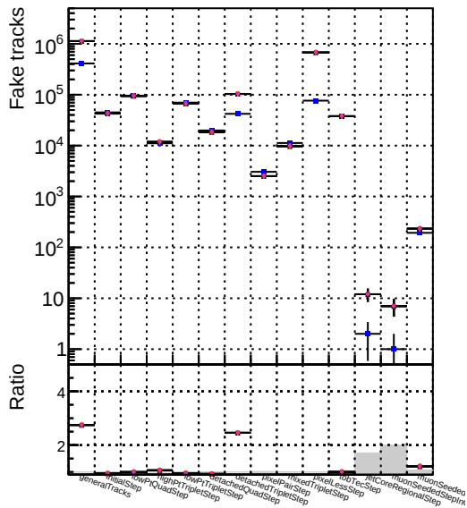
Number Legend Configuration 1 Blue square DOM_CKE_TTbar 2 Red circle DOM_mkFit_TTbarPU-updated 3 Black triangle DOM_mkFit_TTbarPU-updated-newPLDNN 4 Orange star DOM_mkFit_TTbarPU-updated-newPLDNN-2 5 Pink diamond DOM_mkFit_TTbarPU-updated-DNNsqcd13
