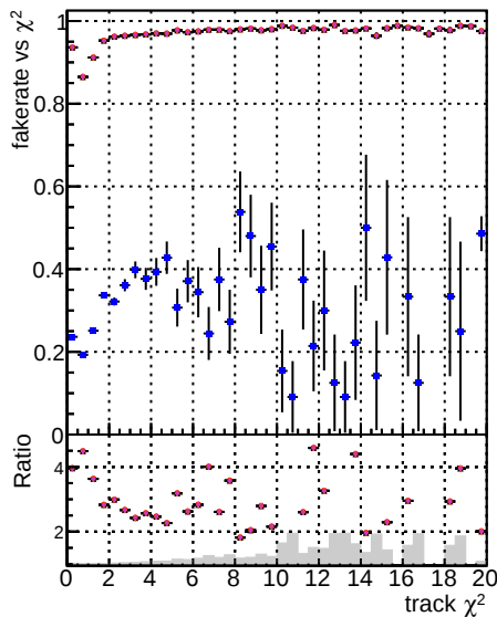
Fake rate vs. DOM GKE TTbar DOM+TTbar GKE+TTbar TTbar+BU-updated newPLDNN DNNsqcd13
