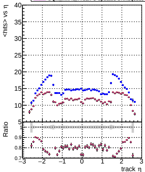
mean hits DOM CKE T1bar DOM mkFit T1barPU-updated DOM mkFit T1barPU-updated-newPLDNN-2 DOM mkFit T1barPU-updated-newPLDNN-3 DOM mkFit T1barPU-updated-DNNsqcd13
