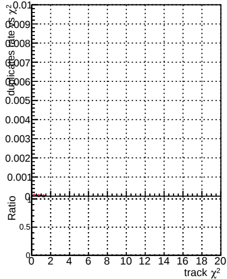
ewPLDNN NNsqc13
