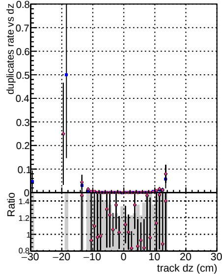
ewBLDNN 2 NNsqcd13
