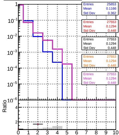
mean hits DOM CKE Tbar DOM mkFit TbarPU-updated DOM mkFit TbarPU-updated-newPLDNN-2 DOM mkFit TbarPU-updated-newPLDNN-2 DOM mkFit TbarPU-updated-DNNsqcd13
