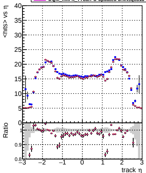
mean hits DOM CKE Tbar DOM mkFit TbarPU-updated DOM mkFit TbarPU-updated-newPLDNN-2 DOM mkFit TbarPU-updated-newPLDNN-2 DOM mkFit TbarPU-updated-DNNsqcd13
