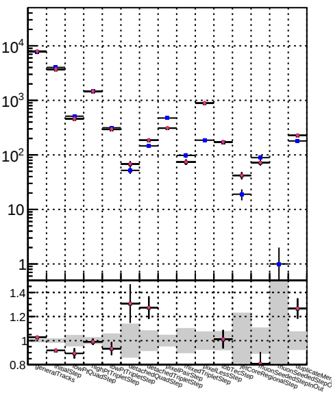
DOM CKE Tbar DOM mkFit TbarPU-updated DOM mkFit TbarPU-updated-newPLDNN DOM mkFit TbarPU-updated-newPLDNN-2 DOM mkFit TbarPU-updated-DNNsqcd13
