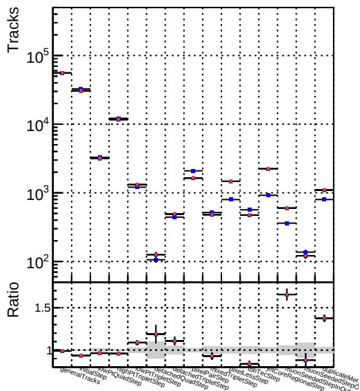
DOM CKE Tbar DOM mkFit TbarPU-updated DOM mkFit TbarPU-updated-newPLDNN DOM mkFit TbarPU-updated-newPLDNN-2 DOM mkFit TbarPU-updated-DNNsqcd13
