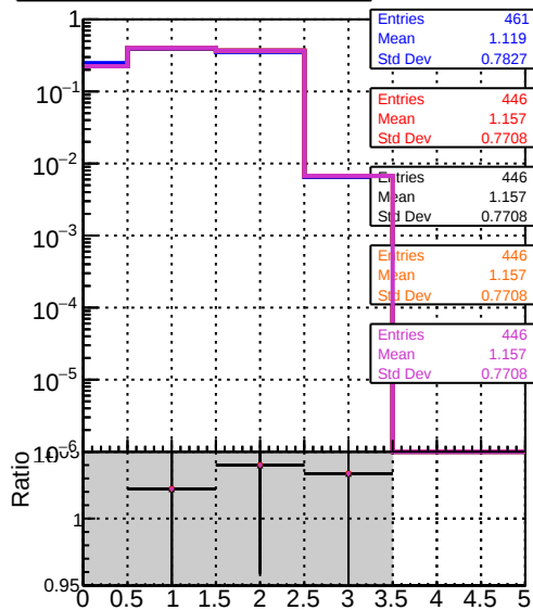
mean hits DOM CKE Tbar DOM mkFit TbarPU-updated DOM mkFit TbarPU-updated-newPLDNN-2 DOM mkFit TbarPU-updated-newPLDNN-2 DOM mkFit TbarPU-updated-DNNsgc113
