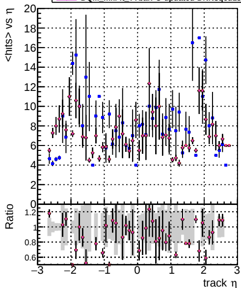
Legend: DOM_CKE_TTbar, DOM_mkFit_TTbarPU-updated, DOM_mkFit_TTbarPU-updated-newPLDNN, DOM_mkFit_TTbarPU-updated-newPLDNN-2, DOM_mkFit_TTbarPU-updated-DNNsqc113 mean hit
