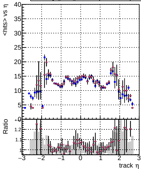
mean hits vs \eta DOM CKE Tbar DOM mkFit TbarPU-updated DOM mkFit TbarPU-updated-newPLDNN-2 DOM mkFit TbarPU-updated-newPLDNN-3 DOM mkFit TbarPU-updated-DNNsqcd13
