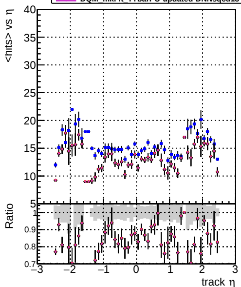
mean hits DOM CKE Tbar DOM mkFit TbarPU-updated DOM mkFit TbarPU-updated-newPLDNN DOM mkFit TbarPU-updated-DNNsgcd13
