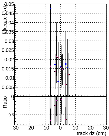
Model Fake rate vs d DOM ~0.05 CKE ~0.05 TTbar ~0.05 DOM+CKE+TTbar ~0.05 PU-updated ~0.05 newPLDNN ~0.05 DNNstd13 ~0.85
