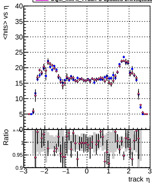
mean hits DOM_CKE_TTbar DOM_mkFit_TTbarPU-updated DOM_mkFit_TTbarPU-updated-newPLDNN DOM_mkFit_TTbarPU-updated-DNNsqc123
