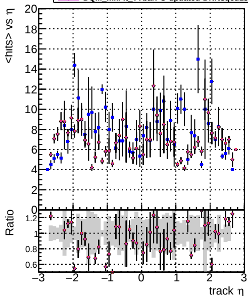
Legend: DOM_CKE_TTbar, DOM_mkFit_TTbarPU-updated, DOM_mkFit_TTbarPU-updated-newPLDNN, DOM_mkFit_TTbarPU-updated-newPLDNN-2, DOM_mkFit_TTbarPU-updated-DNNsqc13 mean hit
