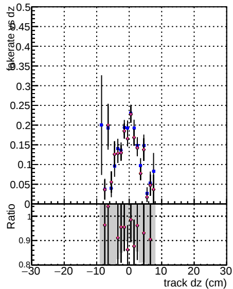
Fake rate vs dz Legend: DOM, GKE, TThar, DOM, MKEL, TThar, BU-updated, DOM, RLNN, 2
