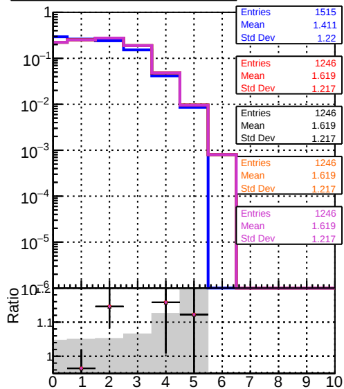
mean hit DOM_CKE_TTbar DOM_mkFit_TTbarPU-updated DOM_mkFit_TTbarPU-updated-newPLDNN-2 DOM_mkFit_TTbarPU-updated-DNNsqcd13
